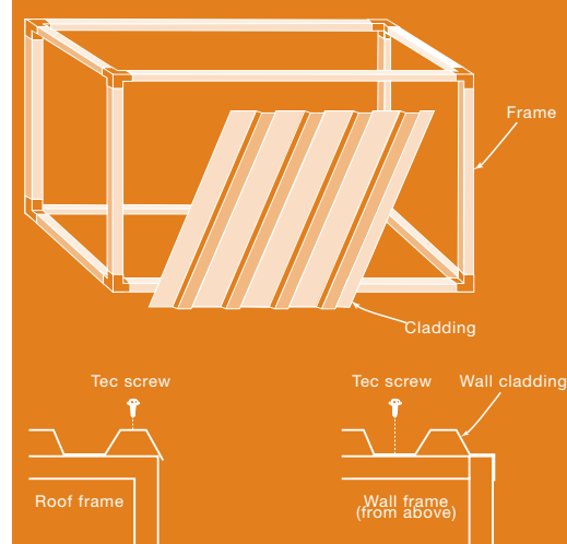
Figure 6: cladding
